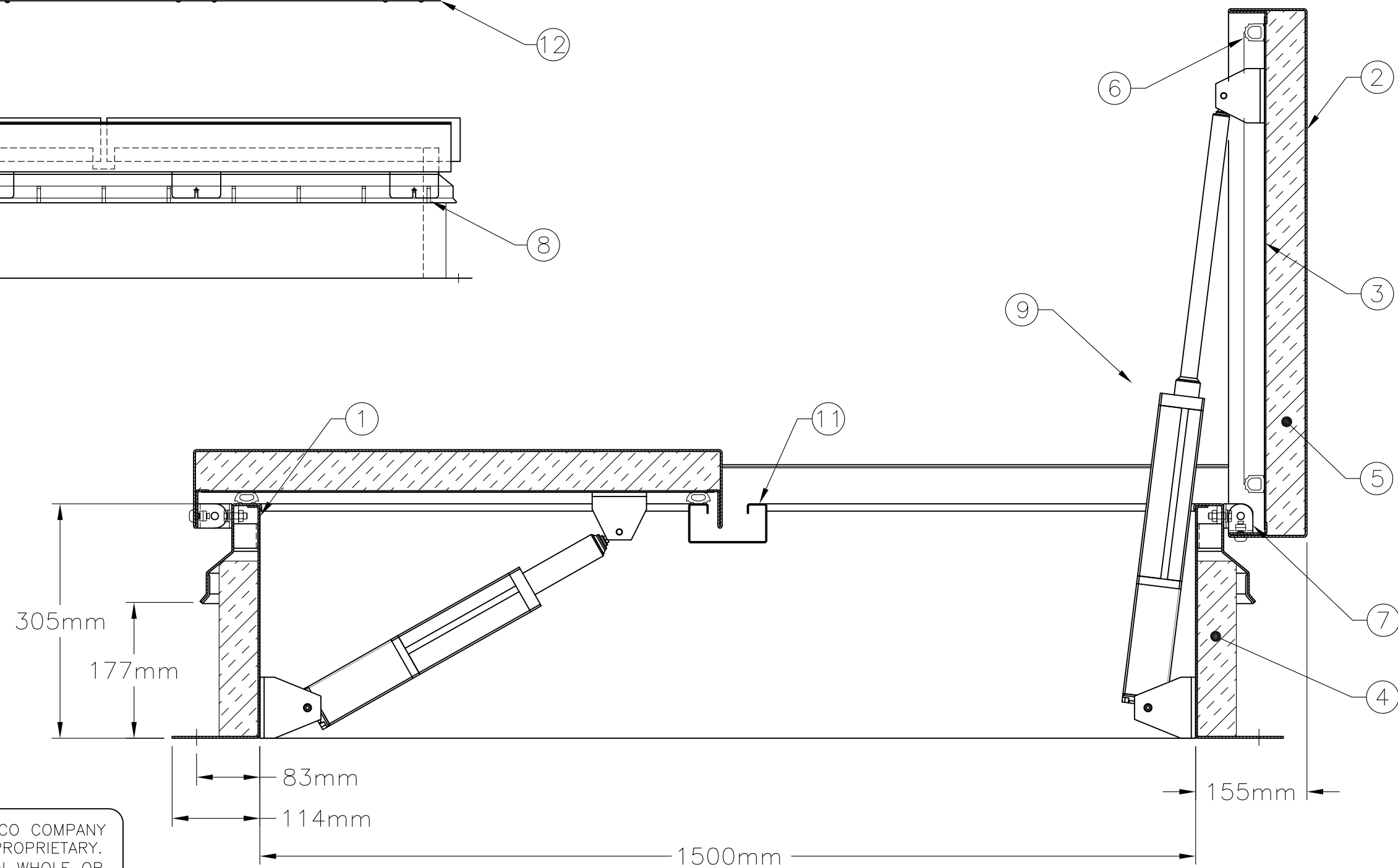
SECTION
