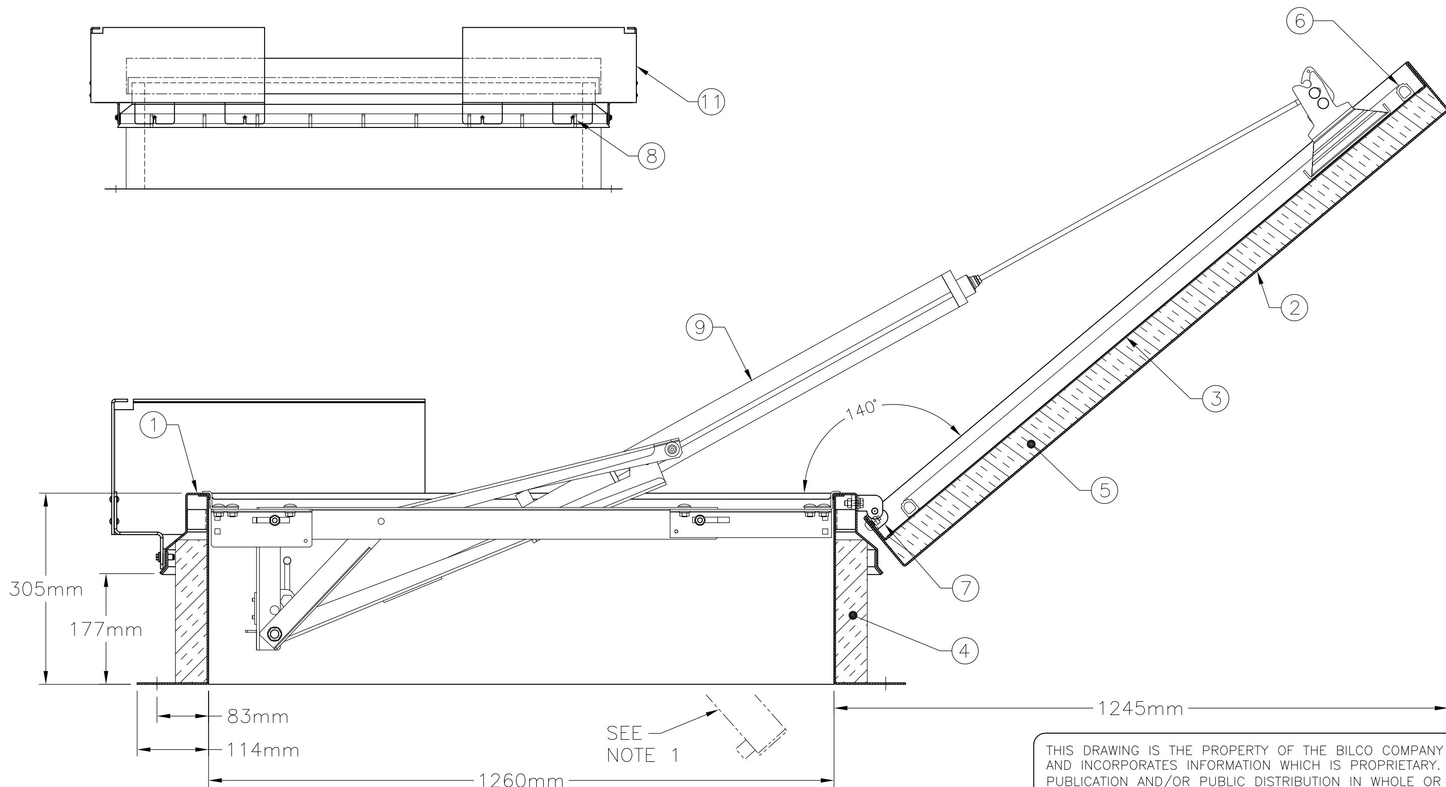
SECTION
